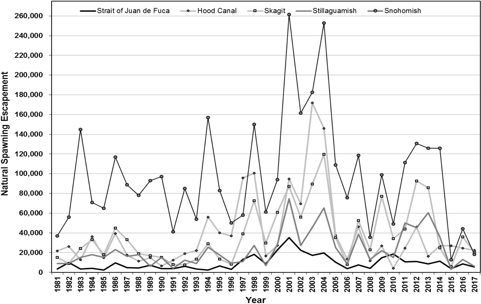
Figure III-4. Puget Sound adult coho natural spawning escapement, 1981-2017.
